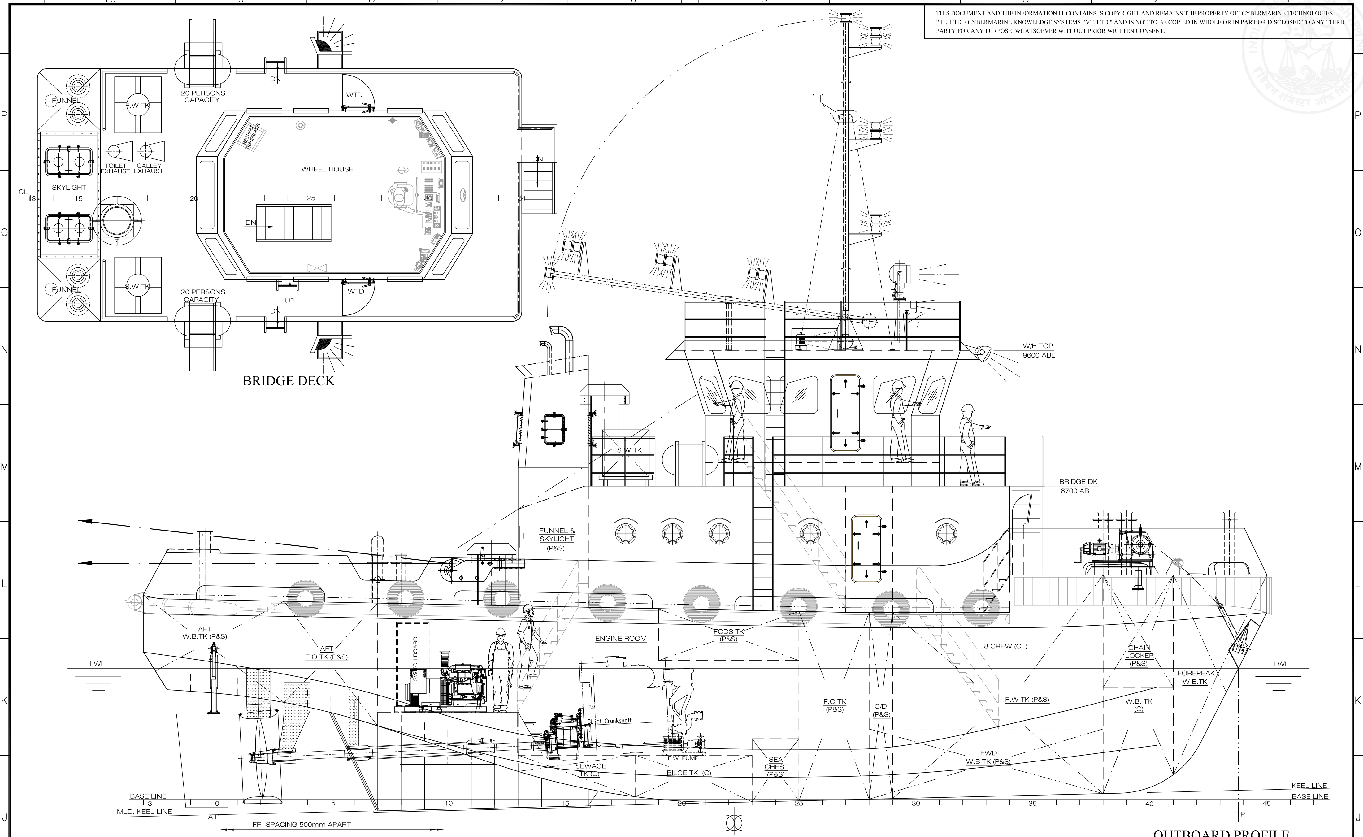
OUTBOARD PROFILE
